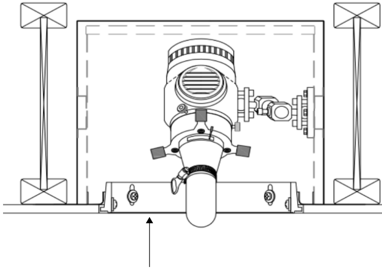
Ceiling Finish Version 1 10" Round Flush Removable Access Cover
