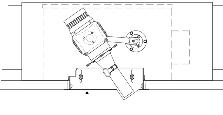
Ceiling Finish Version 2 12" Round Overlap Removable Access Cover
